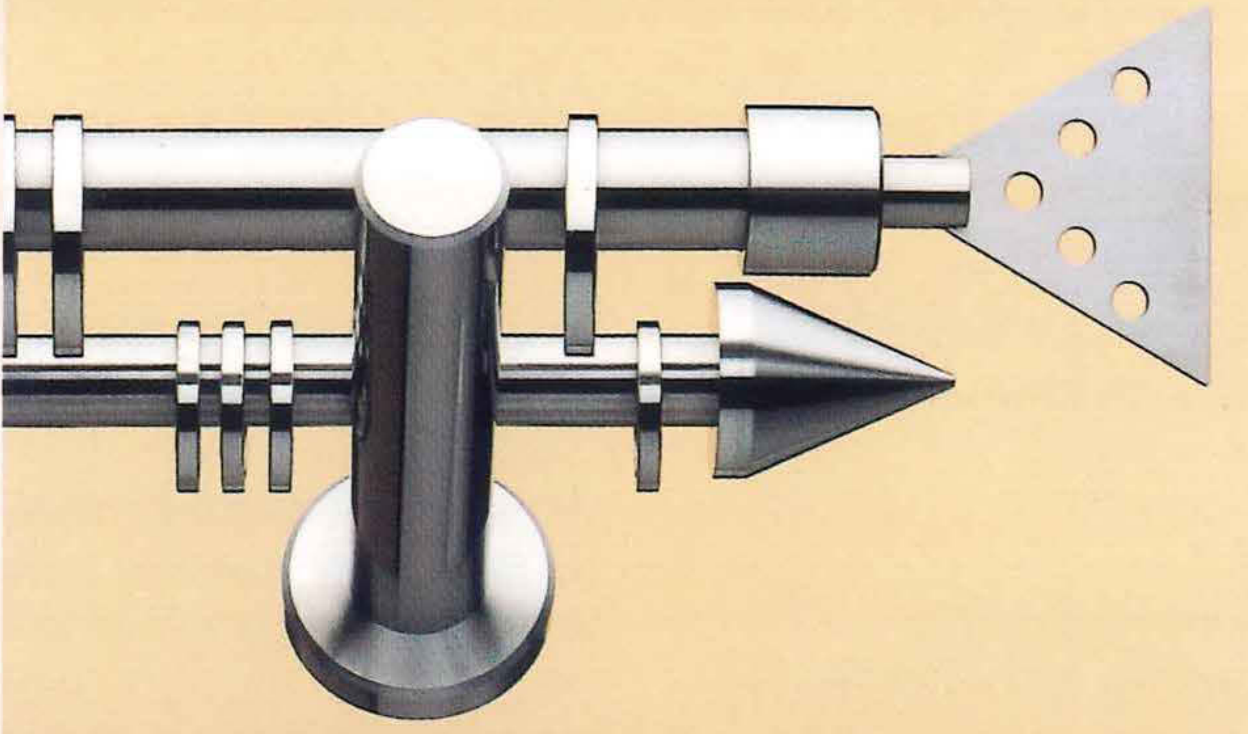
Mod. Budapest - Paris Ø 16 mm, Art. 16.33-11 Abb. Mod. Budapest - Paris Ø 20 mm, Art. 20.33-11 Mod. Budapest - Paris Ø 25 mm, Art. 25.33-11
